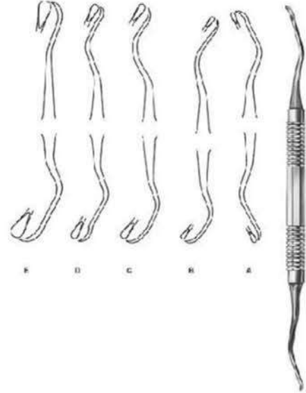
MI-7503 Sinus Lift Curette
